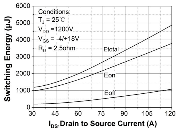
Figure 24. Clamped inductive switching energy vs. drain current ( V_{DD} = 1200\text{V} )
