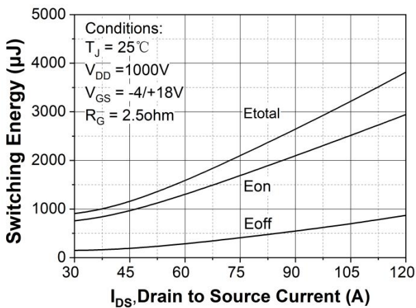
Figure 23. Clamped inductive switching energy vs. drain current ( V_{DD} = 1000\text{V} )
