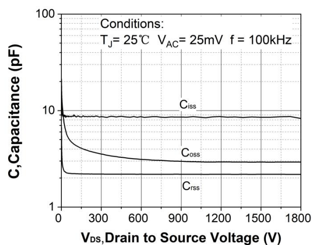
Figure 18. Capacitances vs. drain-source voltage (0 - 1800V)
