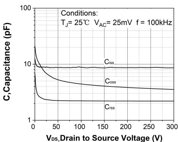
Figure 17. Capacitances vs. drain-source voltage (0 - 300V)
