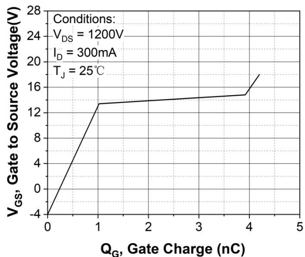
Figure 12. Gate charge characteristic
