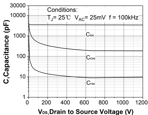
Figure 18. Capacitances vs. drain-source voltage (0 - 1200V)
