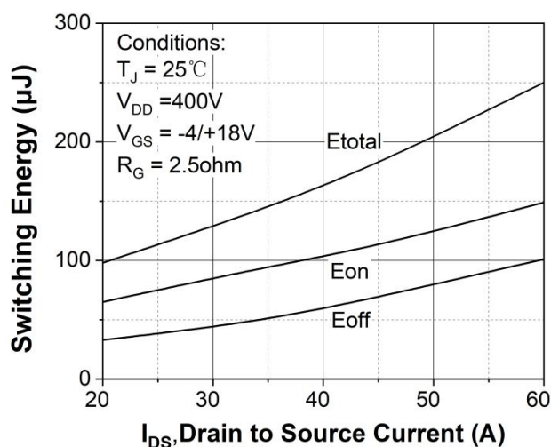
Figure 23. Clamped Inductive switching energy vs. drain current ( V_{DD} = 400\text{V} )
