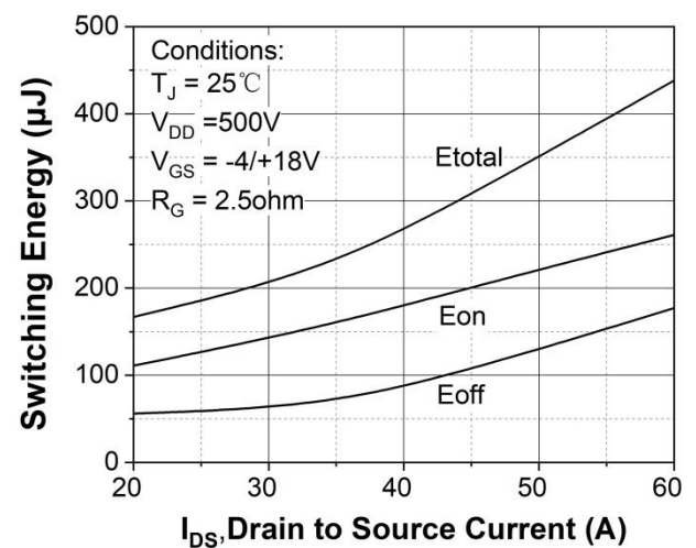
Figure 24. Clamped inductive switching energy vs. drain current ( V_{DD} = 500\text{V} )
