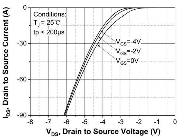
Figure 9. Body diode characteristic at T_J = 25^\circ C
