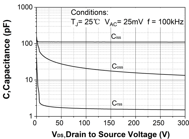
Figure 17. Capacitances vs. drain-source voltage (0 - 300V)
