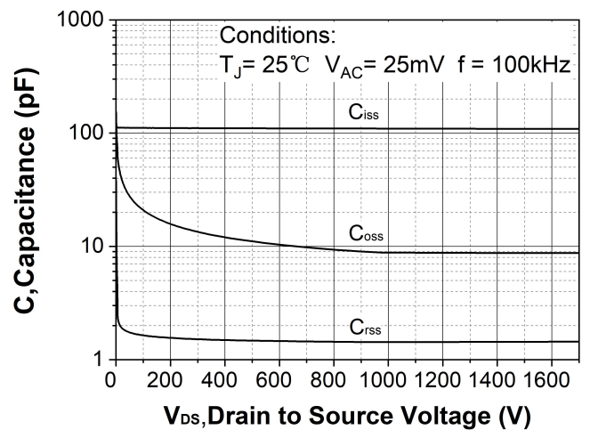
Figure 18. Capacitances vs. drain-source voltage (0 - 1700V)
