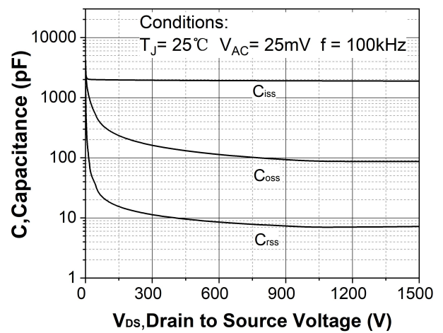
Figure 18. Capacitances vs. drain-source voltage (0 - 1500V)
