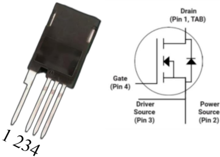
TO-247plus-4L
