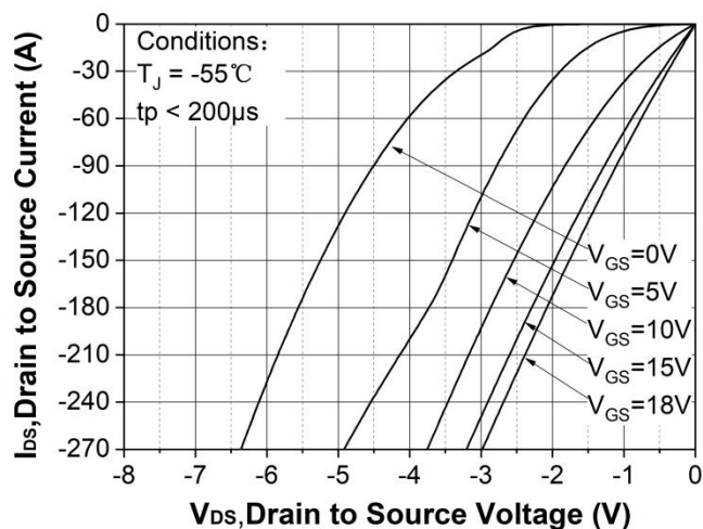
Figure 13. 3rd quadrant characteristic at T_J = -55^\circ\text{C}
