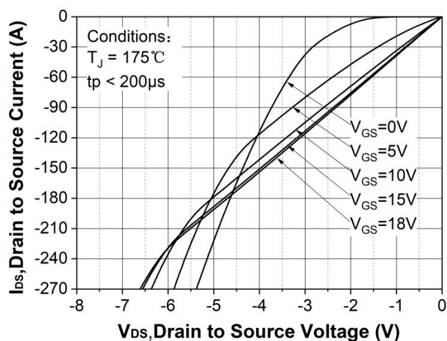
Figure 15. 3rd quadrant characteristic at T_J = 175^\circ\text{C}
