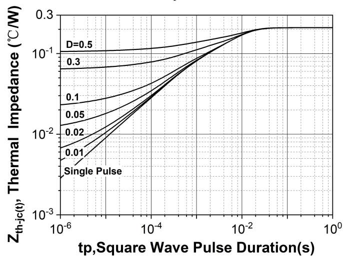
Figure 21. Transient thermal impedance (junction - case)
