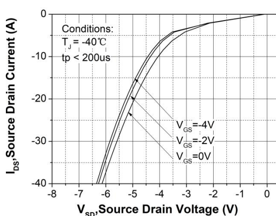
Figure 8. Body diode characteristic at T_J = -40\text{ }^{\circ}\text{C}
