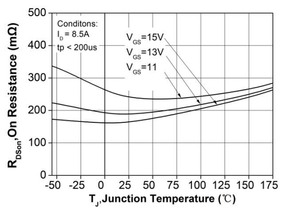
Figure 6. On-resistance vs. temperature for various gate voltages
