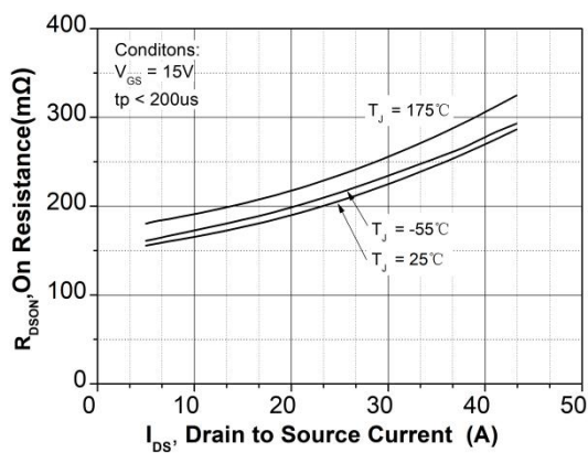
Figure 5. On-resistance vs. drain current for various temperatures
