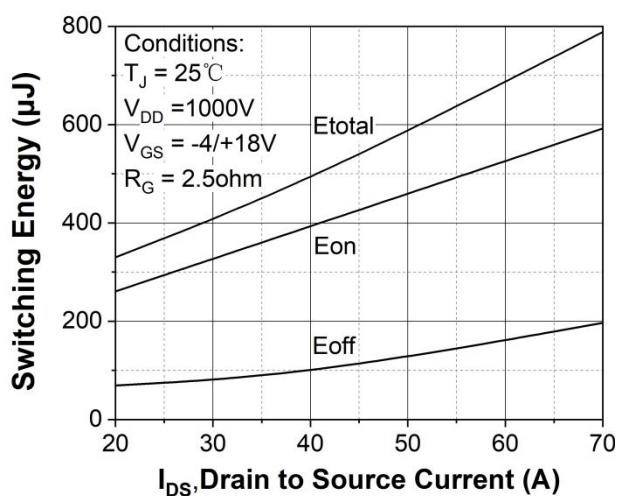
Figure 24. Clamped inductive switching energy vs. drain current ( V_{DD} = 1000\text{V} )
