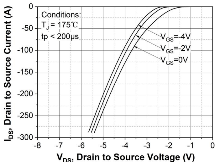
Figure 10. Body diode characteristic at T_J = 175^\circ\text{C}
