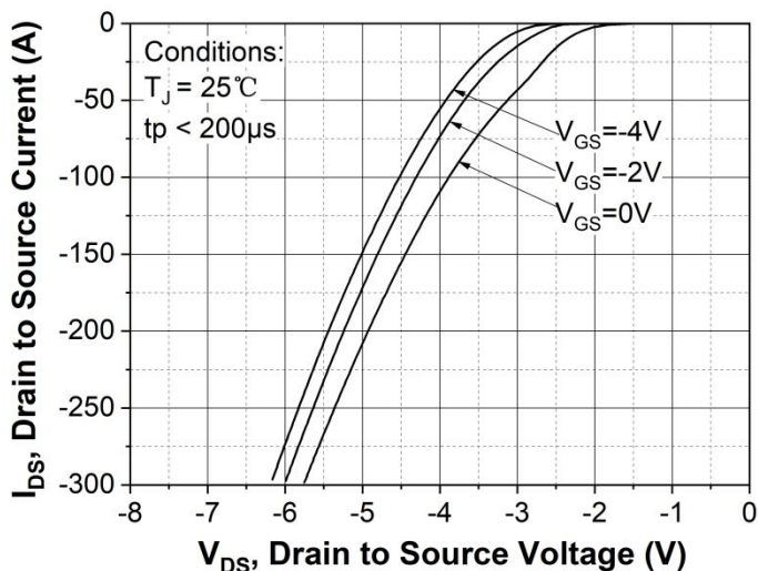
Figure 9. Body diode characteristic at T_J = 25^\circ\text{C}
