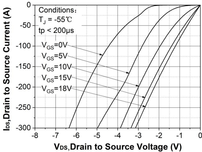
Figure 13. 3rd quadrant characteristic at T_J = -55\text{ }^{\circ}\text{C}
