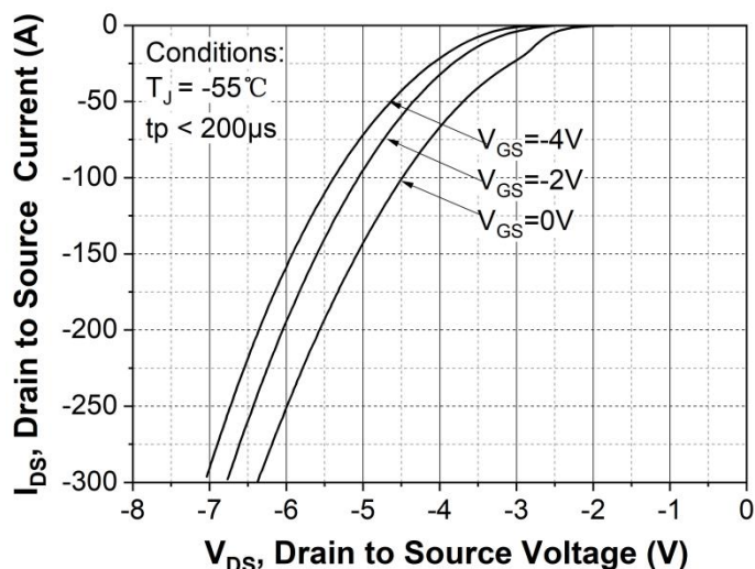
Figure 8. Body diode characteristic at T_J = -55^\circ\text{C}
