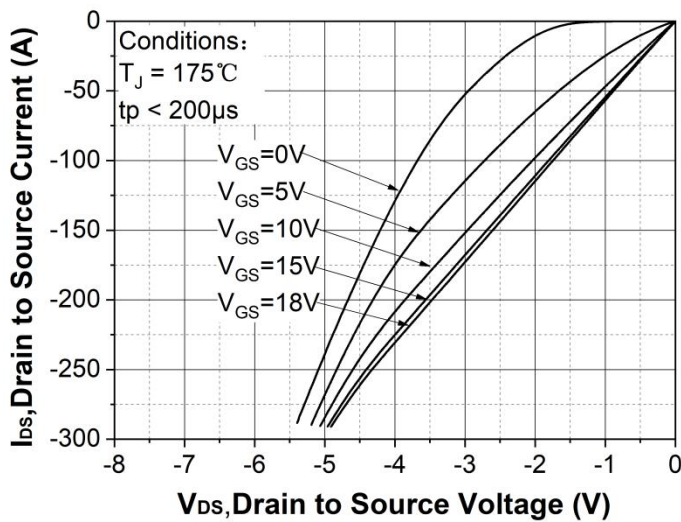
Figure 15. 3rd quadrant characteristic at T_J = 175\text{ }^{\circ}\text{C}
