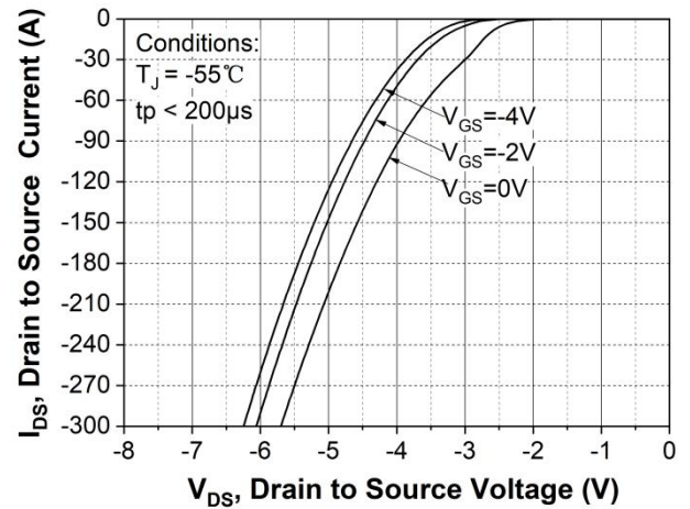
Figure 8. Body diode characteristic at T_J = -55^\circ\text{C}
