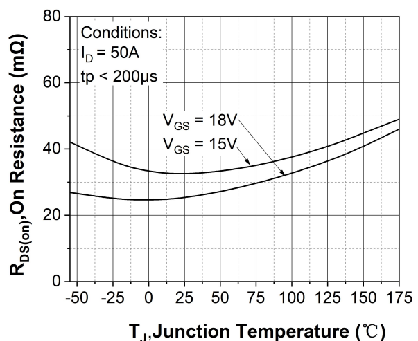
Figure 6. On-resistance vs. temperature for
