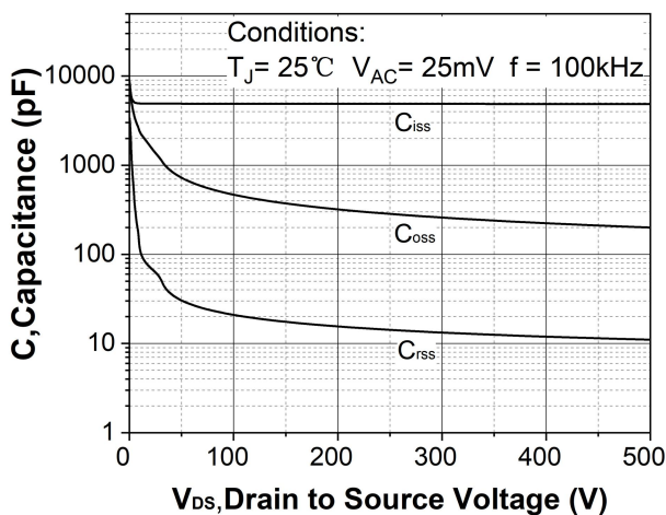
Figure 17. Capacitances vs. drain-source voltage (0 - 500V)
