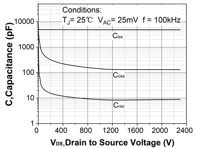
Figure 18. Capacitances vs. drain-source voltage (0 - 2300V)
