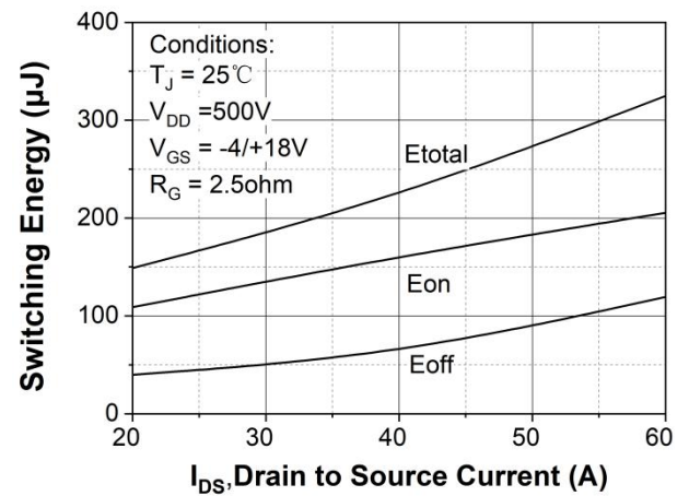
Figure 24. Clamped inductive switching energy vs. drain current ( V_{DD} = 500\text{V} )
