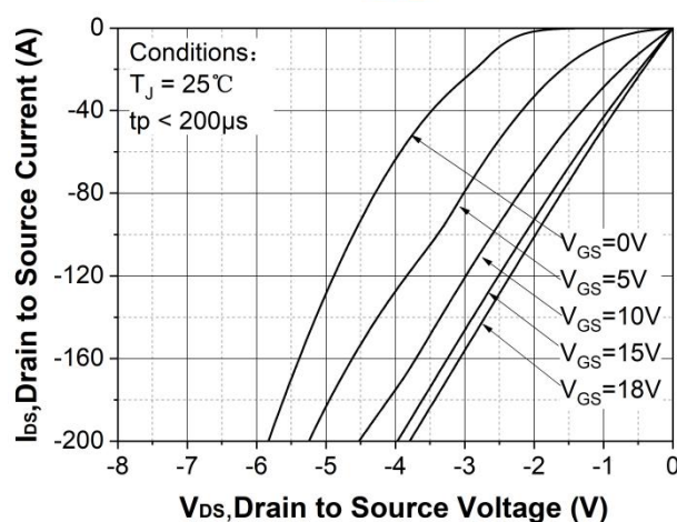
Figure 14. 3rd quadrant characteristic at T_J = 25^\circ\text{C}
