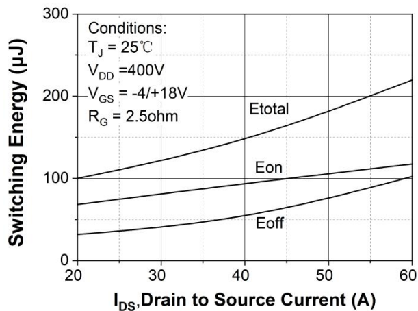
Figure 23. Clamped Inductive switching energy vs. drain current ( V_{DD} = 400\text{V} )
