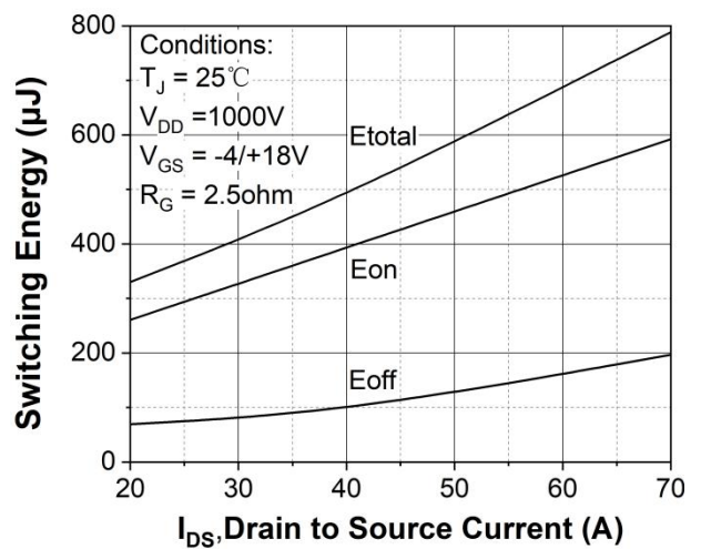
Figure 24. Clamped inductive switching energy vs. drain current ( V_{DD} = 1000V )
