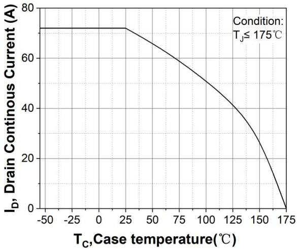
Figure 19. Continuous drain current derating vs. case temperature
