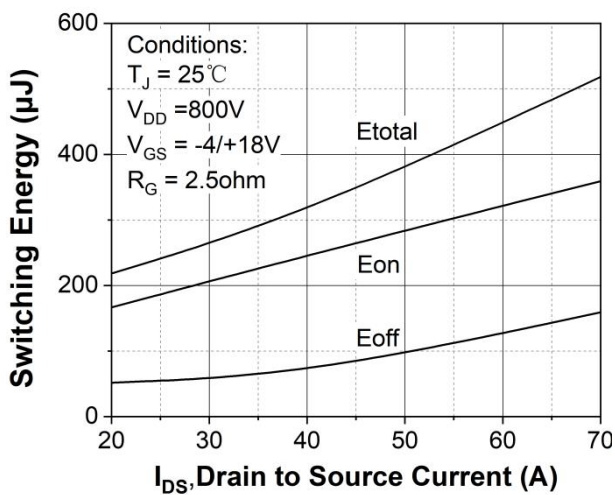
Figure 23. Clamped Inductive switching energy vs. drain current ( V_{DD} = 800V )
