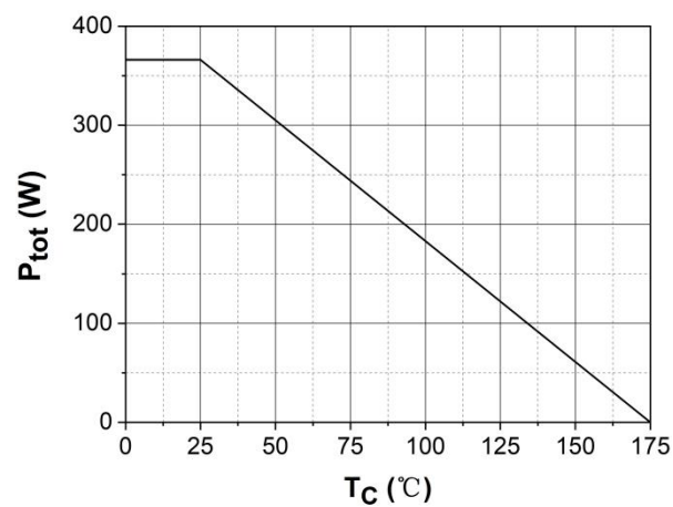
Figure 6. Power Derating
