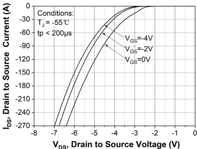
Figure 8. Body diode characteristic at T_J = -55^\circ C
