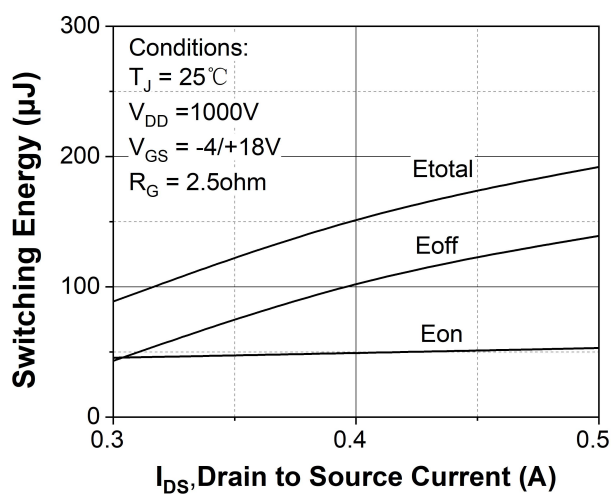
Figure 23. Clamped Inductive switching energy vs. drain current ( V_{DD} = 1000\text{V} )
