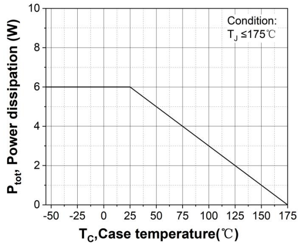
Figure 20. Maximum power dissipation derating vs. case temperature
