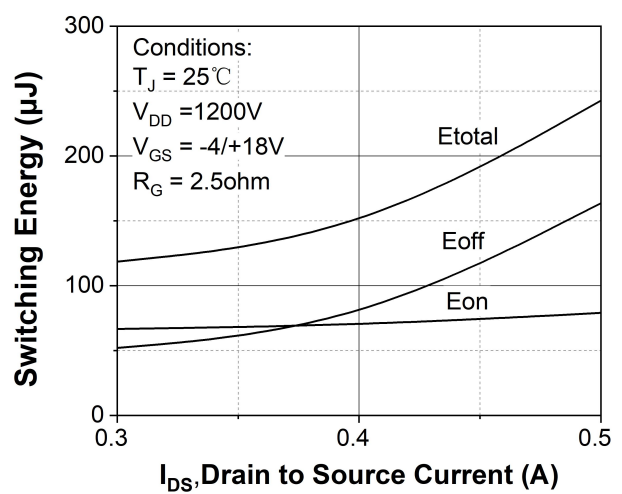
Figure 24. Clamped inductive switching energy vs. drain current ( V_{DD} = 1200\text{V} )
