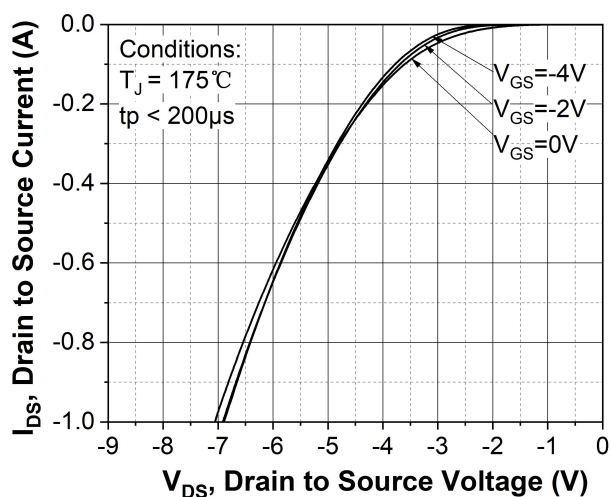
Figure 10. Body diode characteristic at T_J = 175\text{ }^{\circ}\text{C}
