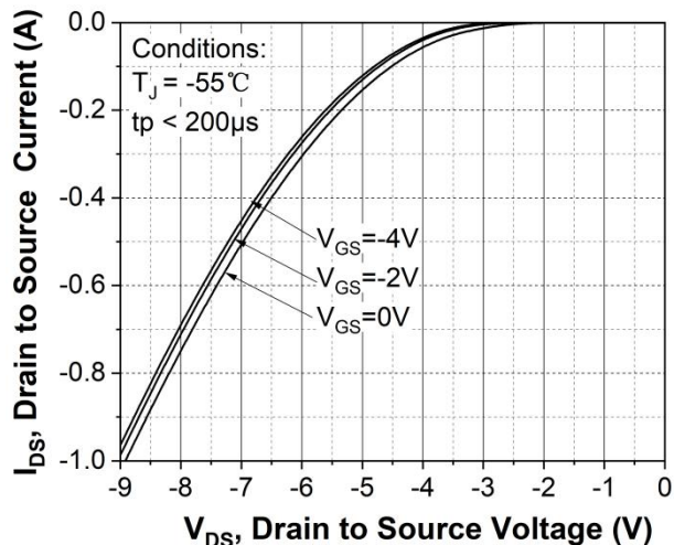
Figure 8. Body diode characteristic at T_J = -55\text{ }^{\circ}\text{C}
