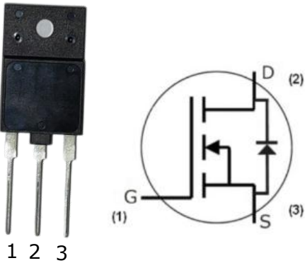
TO-3PF-3L
