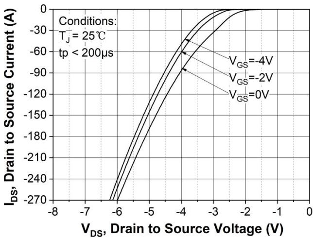
Figure 9. Body diode characteristic at T_J = 25\text{ }^{\circ}\text{C}
