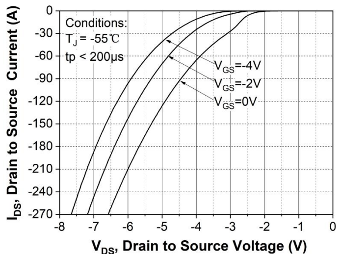
Figure 8. Body diode characteristic at T_J = -55\text{ }^{\circ}\text{C}
