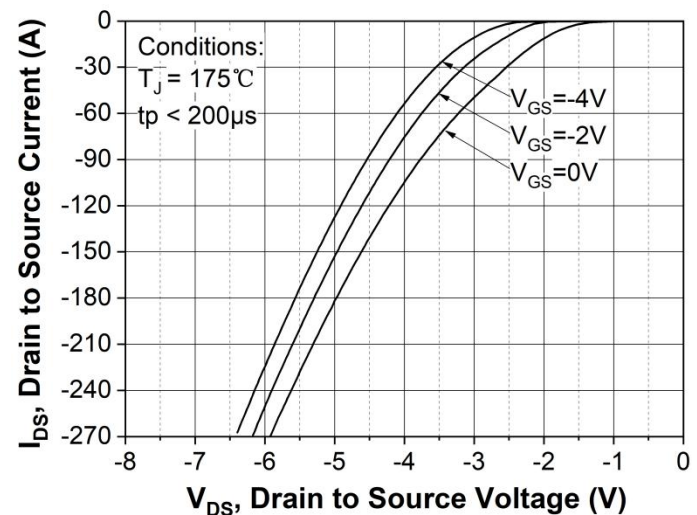
Figure 10. Body diode characteristic at T_J = 175\text{ }^{\circ}\text{C}
