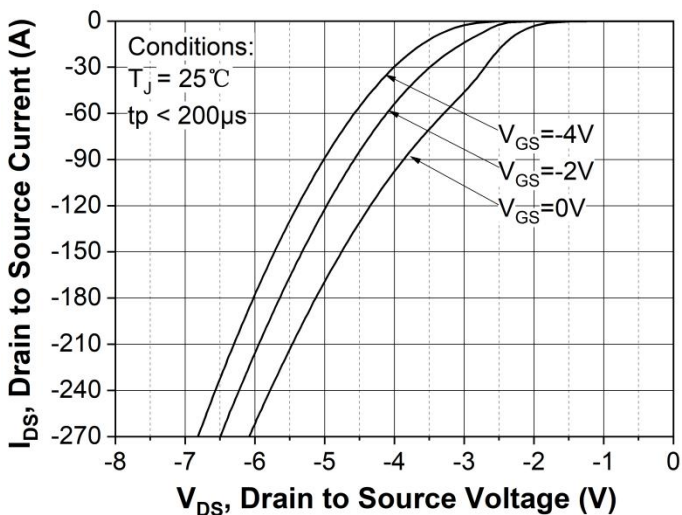
Figure 9. Body diode characteristic at T_J = 25\text{ }^{\circ}\text{C}
