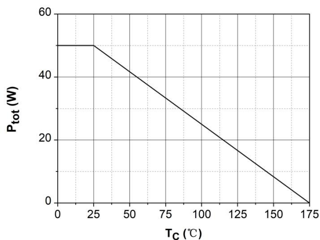
Figure 6. Power Derating
