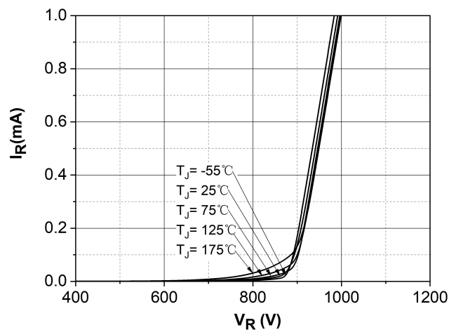
Figure 2. Reverse Characteristics
