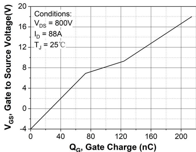
Figure 12. Gate charge characteristic
