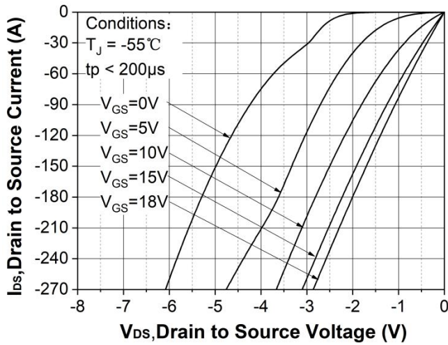
Figure 13. 3rd quadrant characteristic at T_J = -40\text{ }^{\circ}\text{C}
